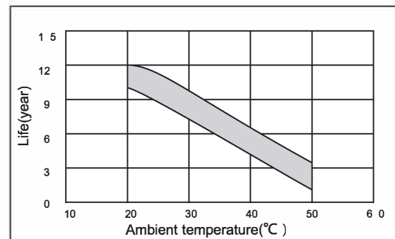
The effect of temperature on float life
