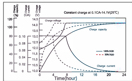
Charging characteristic
